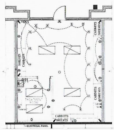
1 PROPOSED POWER, ELECTRICAL, TEL, & DATA PLAN
