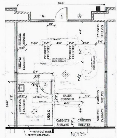
4 PROPOSED FLOOR PLAN
