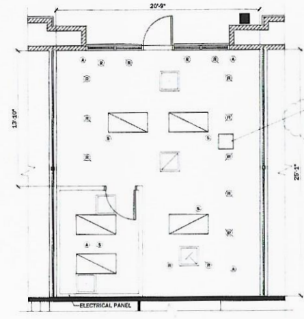
3 PROPOSED RCP
