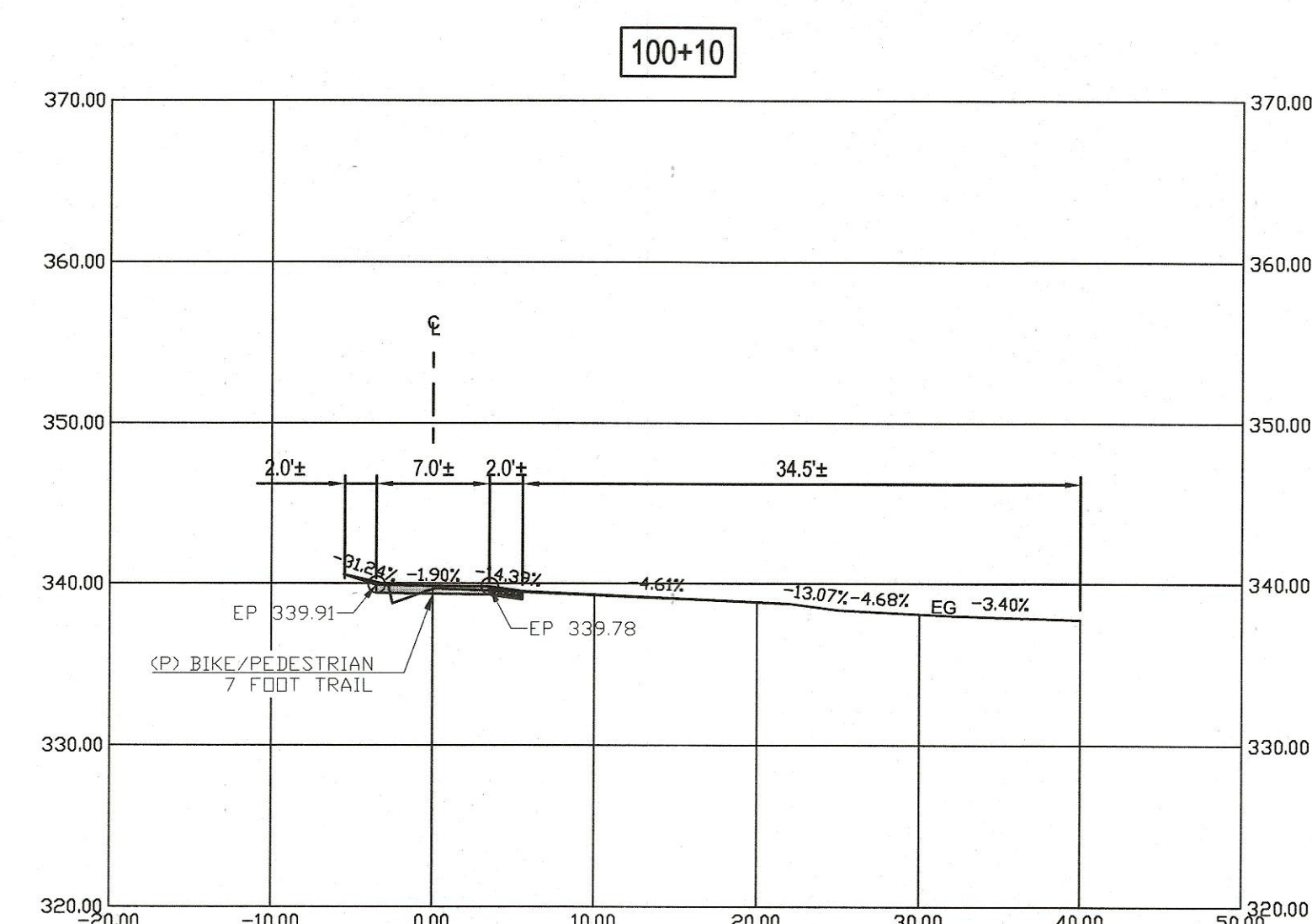
MADRONE CHANNEL TRAIL PHASE 2 - TYPICAL ROAD SECTIONS SCALE: 1" = 10'
