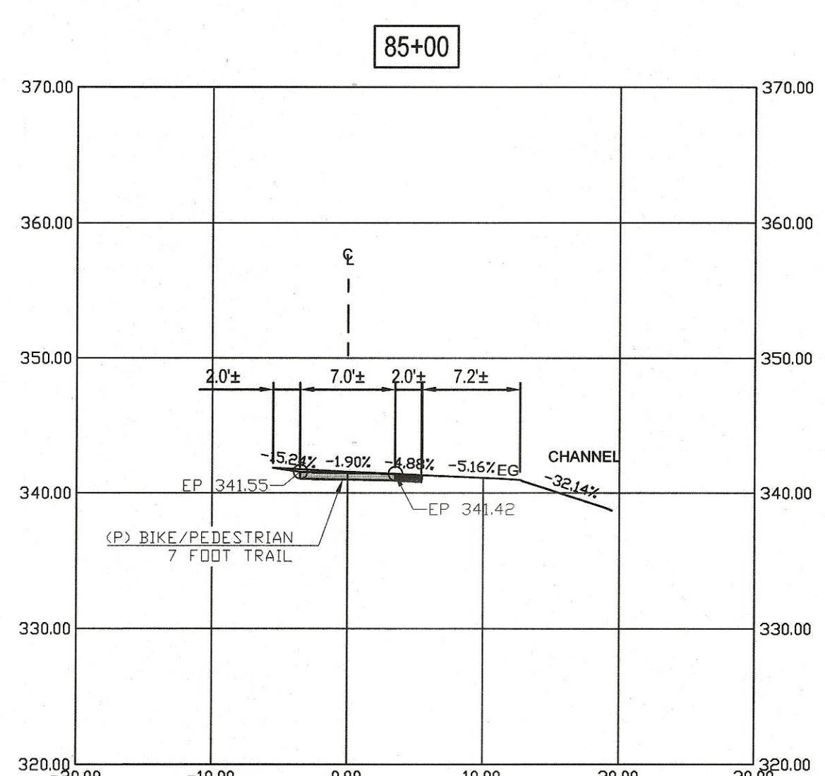
MADRONE CHANNEL TRAIL PHASE 2 - TYPICAL ROAD SECTIONS SCALE: 1" = 10'
